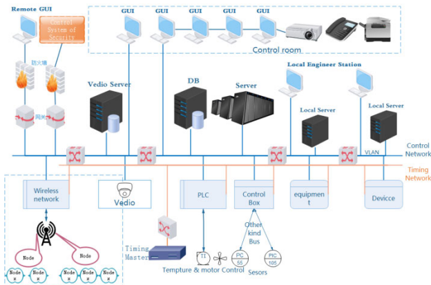
Figure 1: Control system hardware scope of view.
