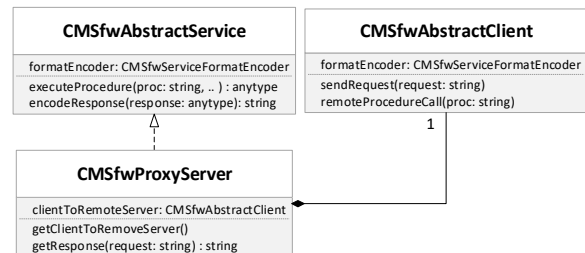
Figure 2: Service-client composition.
