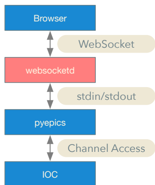
Figure 2: Principle of the status push program.
