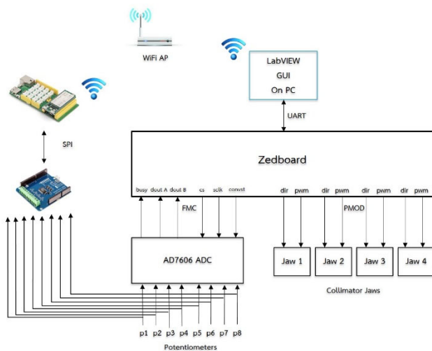
Figure 9: System block diagram of the updated system.
