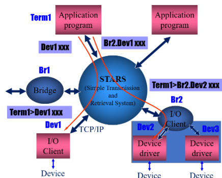
Figure 1: Message transportation on STARS.*
