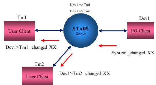
Figure 3: Event delivery function of STARS.*
